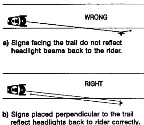
Figure 2 - Sign Orientation, Plan View
