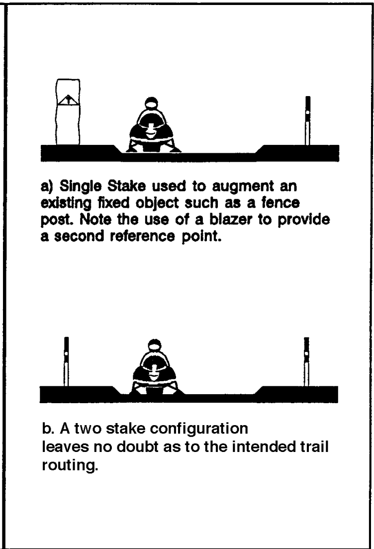
Figure 5 - Examples of Staking
